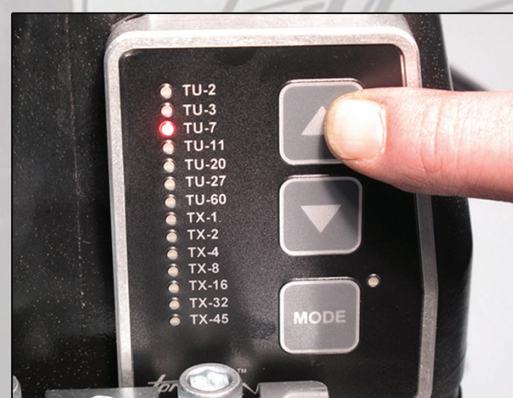
Push button tool selection for Torcup TU and TX Wrenches
